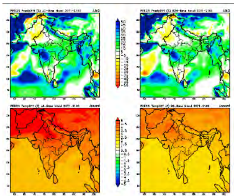
Figure 4 Projected changes in summer monsoon precipitation and surface air temperature by 2100 under A2 and B2 scenarios of PRECIS model derived from HadCM3.
