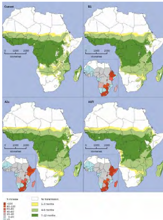
Figure 2: Plasmodium falciparum malaria transmission
