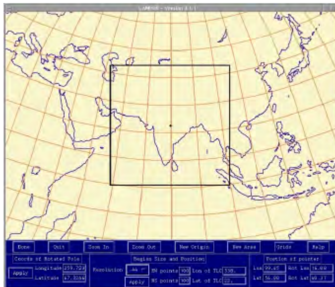
Figure 3. Coverage by PRECIS runs at IITM, Pune
