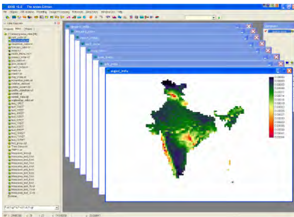
Figure 5 Monthly rainfall data files from PRECIS model in GIS format
