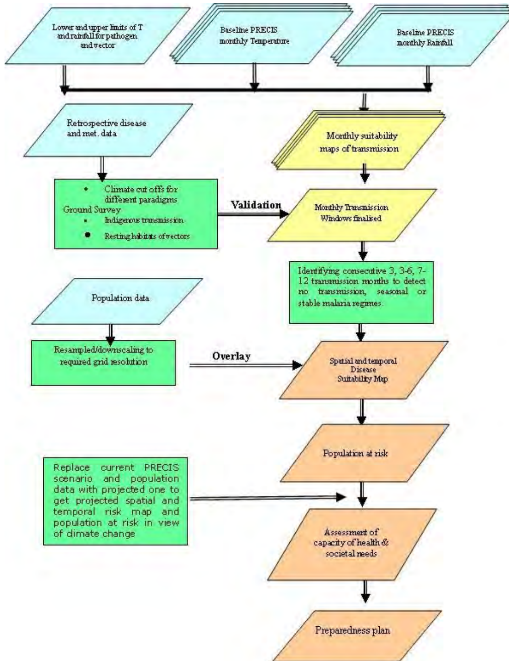
Figure 6: Generic framework for assessment of impact of climate change on vector-borne diseases
